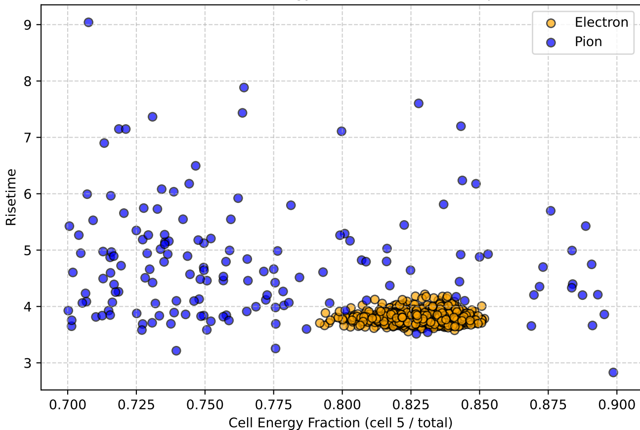
Risetime vs Cell Energy Fraction for 60.0GeV particles
